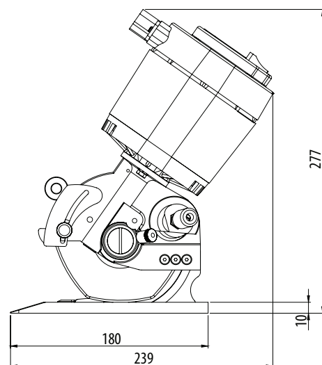
Dimension layout
