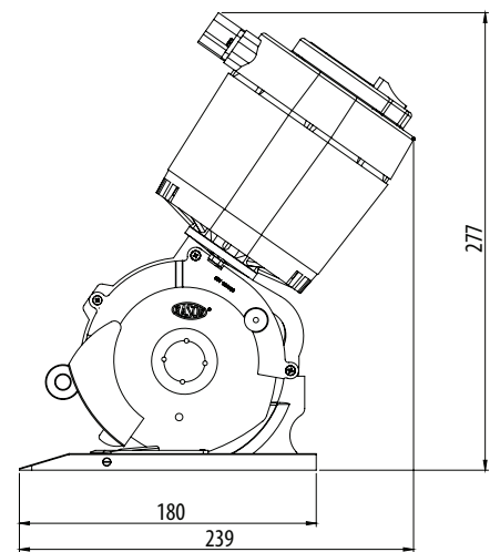
Dimension layout
